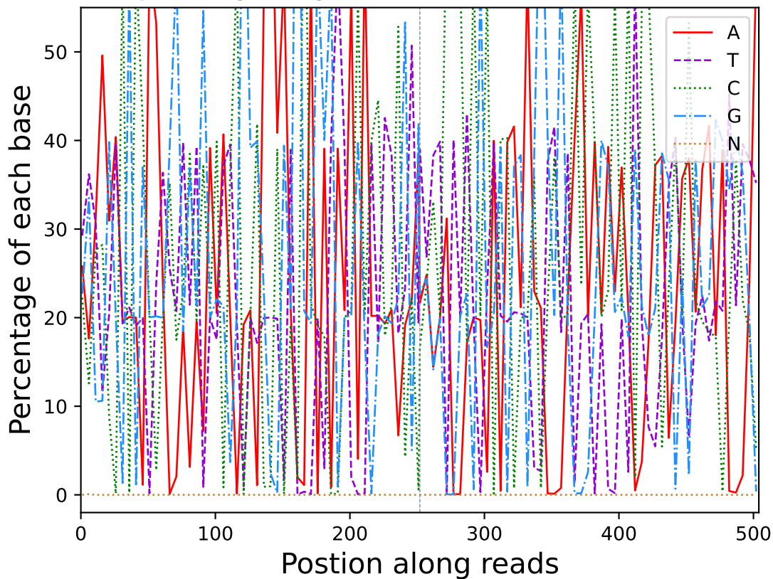
Base percentage along reads (R10702)
